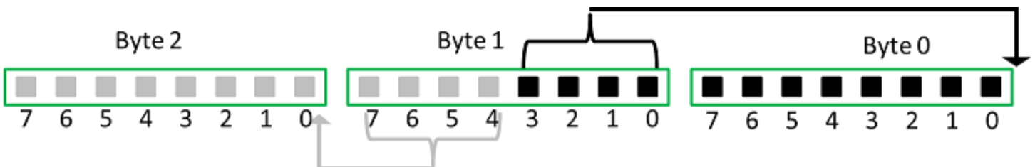
Figure 2. Packing two 12-bit pixels into three bytes.
